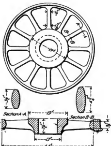
Figs. 3541-3544. 44-Inch Trailing Truck Wheel Center. American Locomotive Co.
